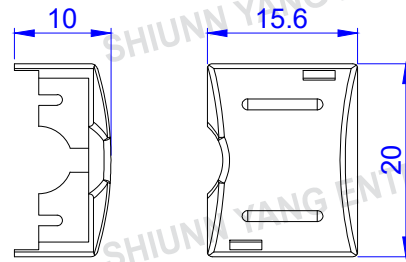
ENCLOSURE IDC CAP x 1 PC
