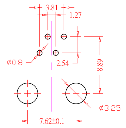
PCB LAYOUT
